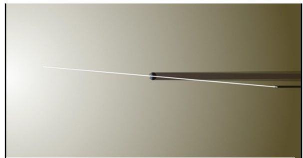
Figure 4 Depiction showing Moon's orbit 5 degrees inclined to Earth's with their respective shadows trailing into space. Courtesy, NASA https://solarsystem.nasa.gov/moons/earths-moon/lunar-phases-and-eclipses/
