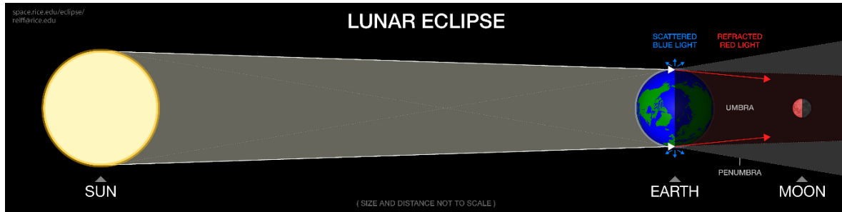
Figure 5 Rice Space Institute graphic showing how a lunar eclipse occurs as Earth's shadow coincides with the Moon's orbital path. https://space.rice.edu/eclipse/img/eclipse_diagram_lunar.jpg
