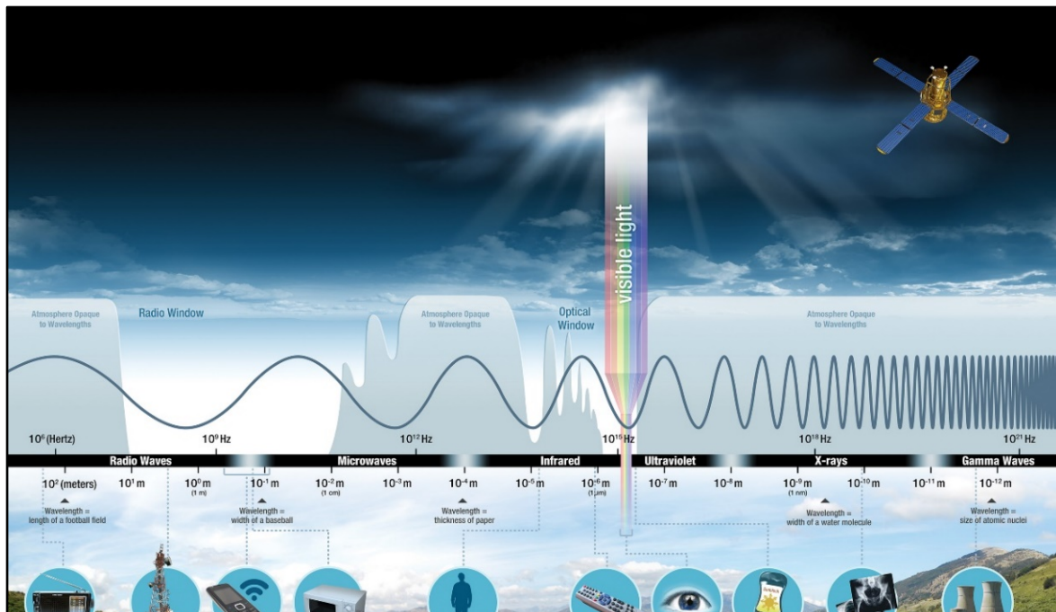
Figure 2 Graphic depicting the range of electromagnetic radiation emitted by the Sun Courtesy NASA, https://www.nasa.gov/analog/nsrl/why-space-radiation-matters
